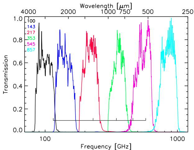
Fig. 15. Bandpasses of HFI with the location of bright CO rotational lines ( J = 1 \rightarrow 0 , 2 \rightarrow 1 , 3 \rightarrow 2 , 4 \rightarrow 3 , and 5 \rightarrow 4 from left to right) shown as a horizontal black line with tick marks. The CO lines can introduce a significant positive bias in the flux density of the sources, particularly those associated with Galactic star-forming regions. The effect is the most significant at 100 GHz where the flux density may be boosted by more than 50%. See Planck HFI Core Team (2011b) for details.
