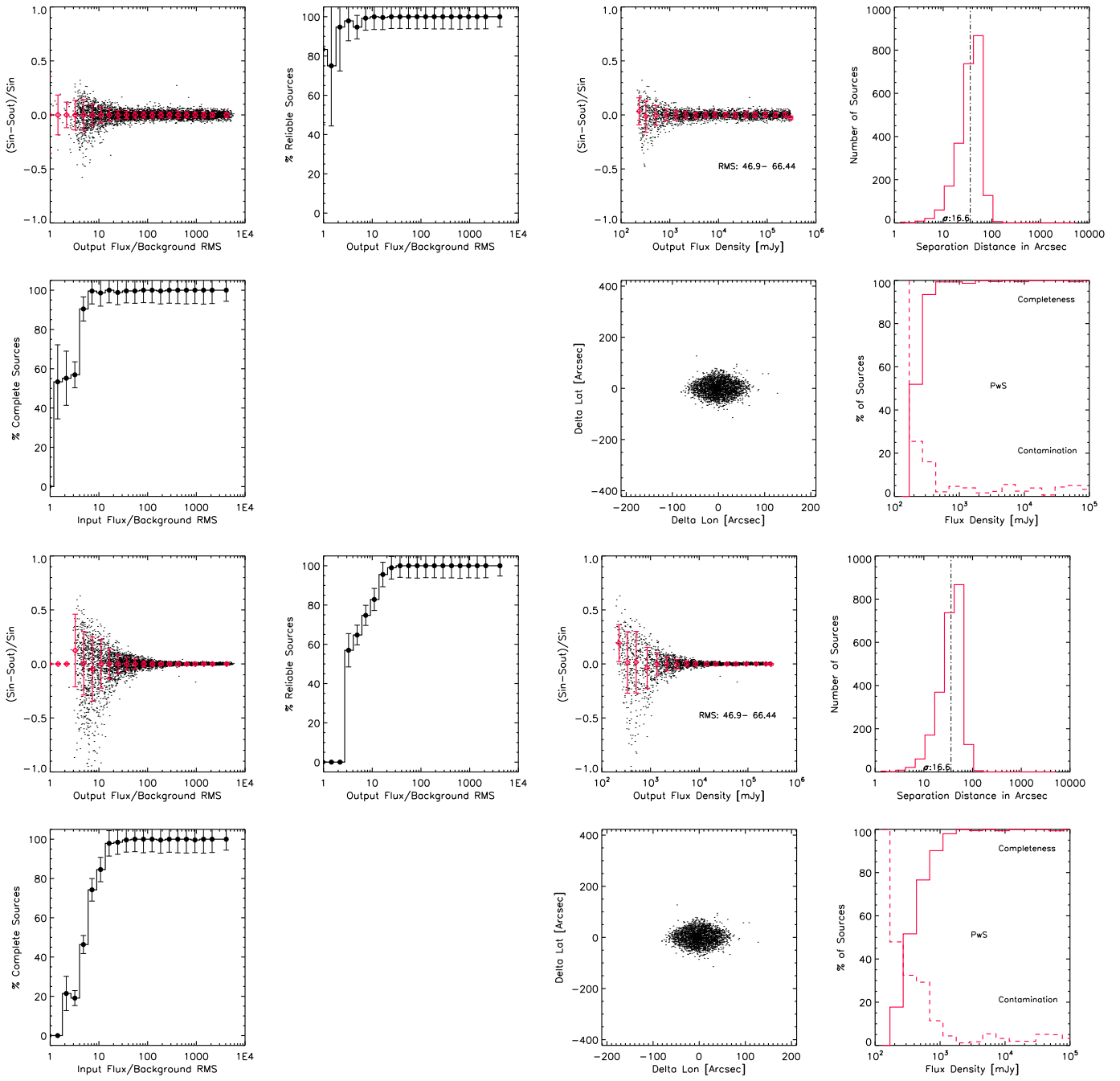
Fig. 3. As in Figure 2 but at 143 GHz with the PwS algorithm.
