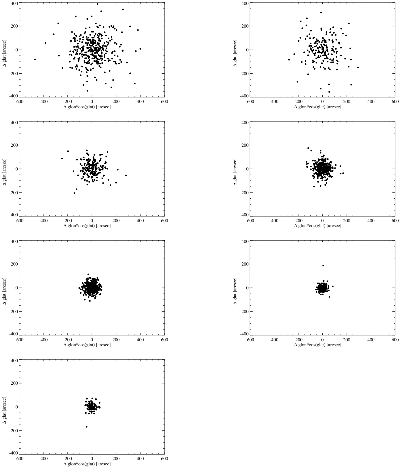
Fig. 10. Matches to quasars as a measure of positional offsets in the ERCSC 30 to 353 GHz catalogues. The top row shows 30 and 44, the second row 70 and 100, the third row 143 and 217, and the final row 353 GHz. There are insufficient numbers of detected quasars at the upper HFI frequencies.
