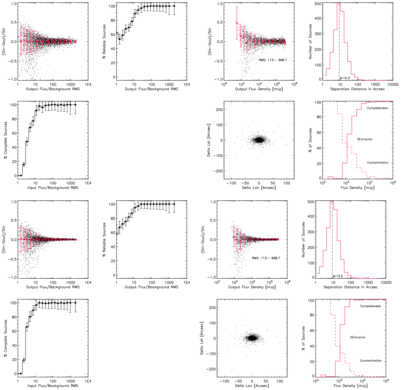
Fig. 4. As in Figure 2 but at 857 GHz with the SExtractor algorithm.
