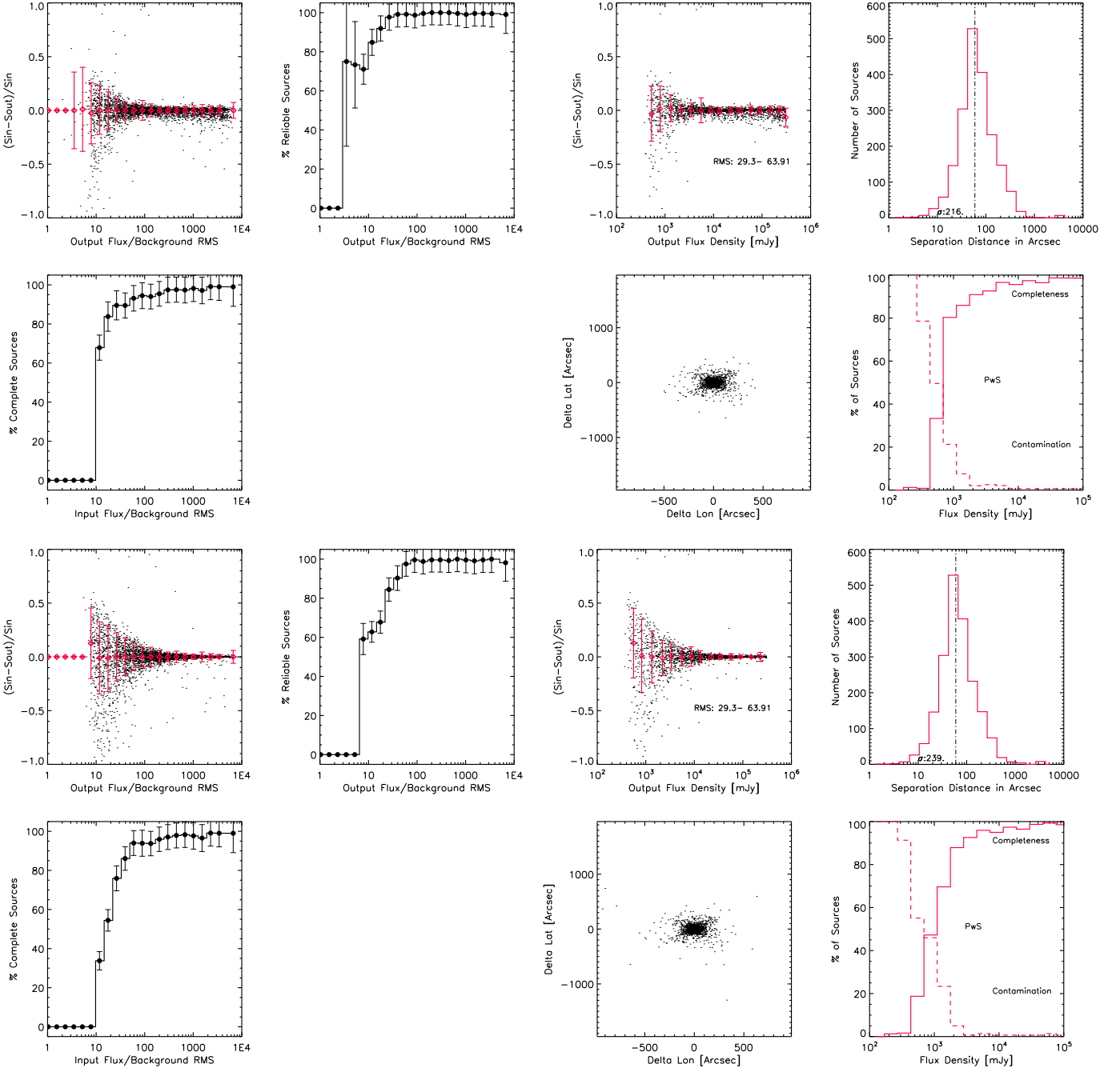
Fig. 2. Plots showing the results of the Monte-Carlo analysis at 30 GHz with the PwS algorithm. The upper two rows shows the results when the flux density of sources is from FLUXDET while the lower two rows shows the results when the flux density of sources is from FLUX. The set of 3 plots in the top-left and bottom-left corner show the all-sky flux-density uncertainty, differential reliability and differential completeness of the Monte-Carlo sources as a function of SNR where signal may be FLUX or FLUXDET and the noise is the background RMS. The set of four plots at the top right and bottom right show (left to right, top to bottom) the fractional flux density uncertainty, (S_{in} - S_{out})/S_{in} (see Sect. 5.1), the distribution of the absolute positional offset, differential positional offset, as well as completeness and contamination (1–reliability converted to a percentage) as a function of flux density for the half of the sky with the lowest sky background RMS. The range of sky background RMS converted to a point source flux density uncertainty, is shown in the inset in mJy. The primary source selections in the catalogues are based on the reliability vs output flux density/background RMS plots such that the cumulative reliability (integral of the differential reliability) is greater than 90%.
