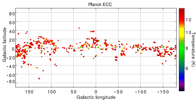
Fig. 18. Sky distribution of ECC detections having \text{SNR} \geq 15 and T \leq 14 K is shown. The symbols are colour-coded by temperature using the scale shown on the right.
