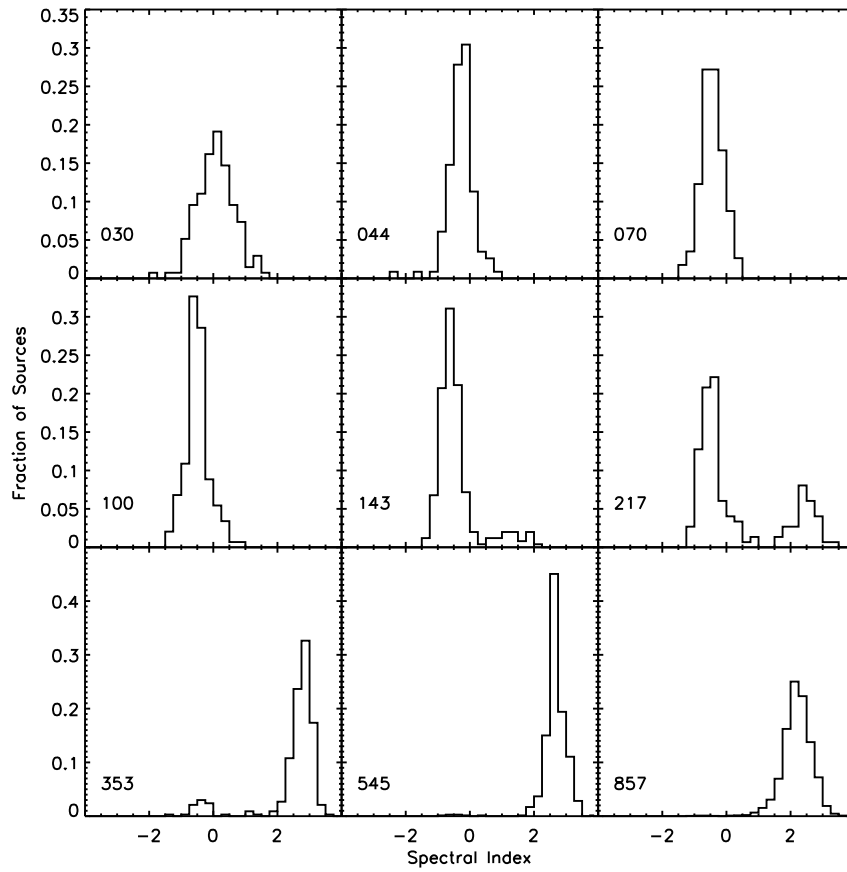
Fig. 8. The distribution of spectral indices for sources above 30^\circ of the Galactic Plane, likely to be dominated by extragalactic sources.
