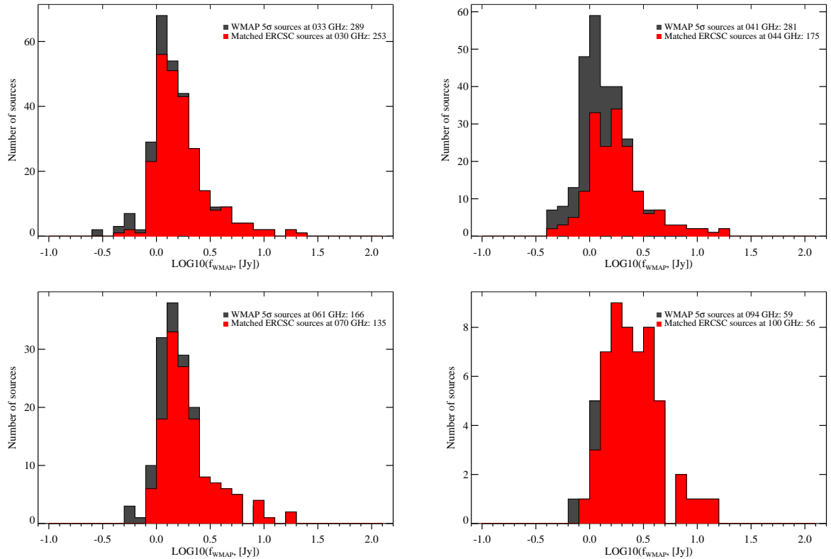
Fig. 12. Histogram distribution of WMAP flux densities for all WMAP 5\sigma sources in each band (gray region). The sources that are detected in the ERCSC are shown as the red histogram. Some of the WMAP sources have been missed because of source variability.
