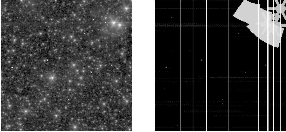
Figure 9: The band 1 (GLIMPSEI) IRAC frame (AOR 12110848, exposure 11) is on the left (corrections were applied for muxbleed and column pulldown); the flags for that frame are shown on the right. Stray light masks (SQF bit 17) are seen in the upper right hand corner of the frame. The PSF-shaped areas around the bright sources correspond to SQF bit 20. The vertical lines correspond to where the frame was corrected for column pulldown (SQF bit 15). The horizontal dots show which pixels were corrected for muxbleed (SQF bits 7 and/or 9). Various small dots are hot, dead or bad pixels (SQF bit 8). Bits in the SQF will have been set for sources within 3 pixels of any of these areas.
