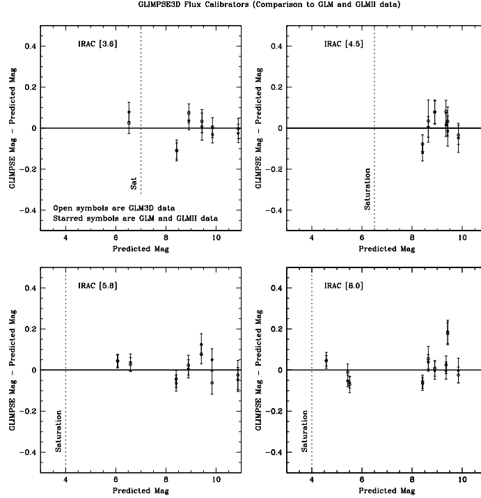
Figure 5: This figure shows the agreement between the GLIMPSE3D extracted magnitudes and the GLIMPSE/GLIMPSEII extracted magnitudes. It confirms that multi-epoch extractions for these stars agree well from epoch to epoch and that the deviations from the predicted magnitudes may be real in some cases.
