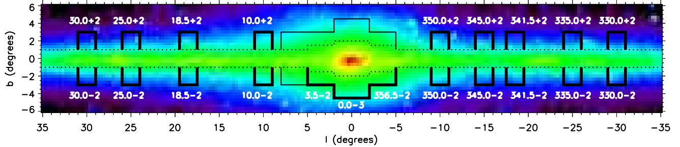
Figure 1: COBE/DIRBE 4.9 \mu\text{m} map of infrared intensity in the Galactic plane. Dotted lines show the area already observed by GLIMPSEI and GLIMPSEII. The vertical extensions for GLIMPSE3D are shown with solid lines. The 21 areas for which mosaics have been provided in the data releases are annotated. Source lists for the entire survey area have been delivered.
